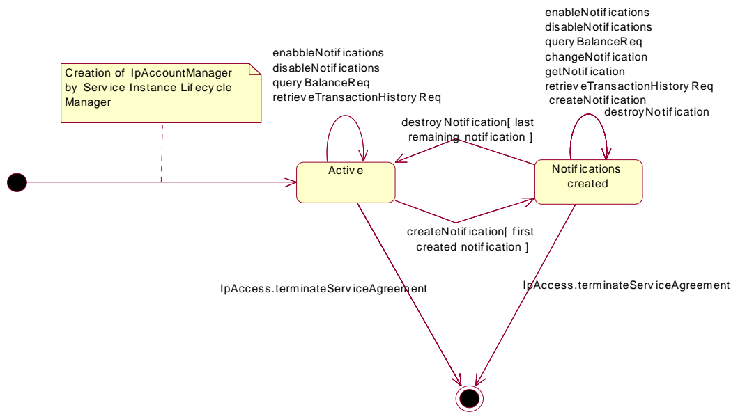
Figure : Application view on the IpAccountManager
