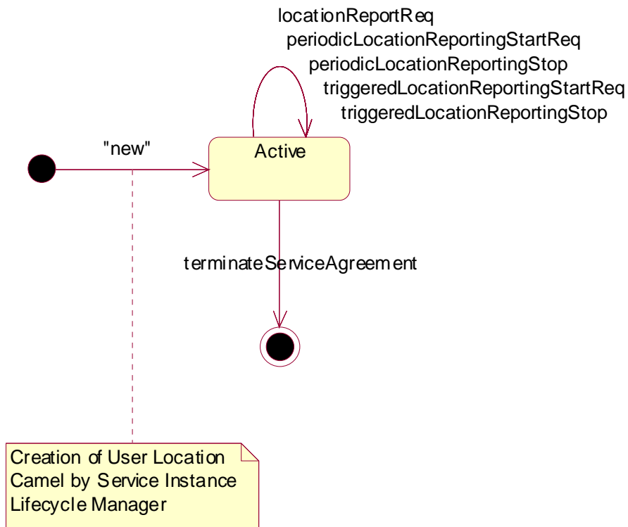
Figure : State Transition Diagram for User Location Camel
