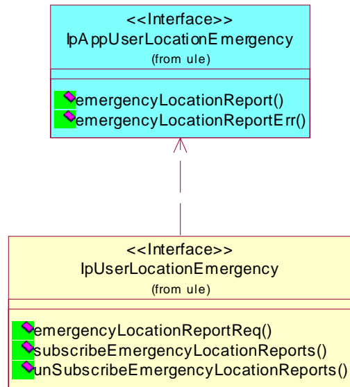
Figure: User Location Emergency Class Diagram
