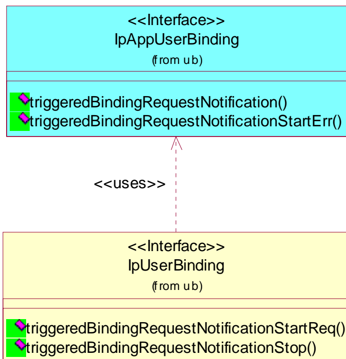
Figure : User Binding Class Diagram
