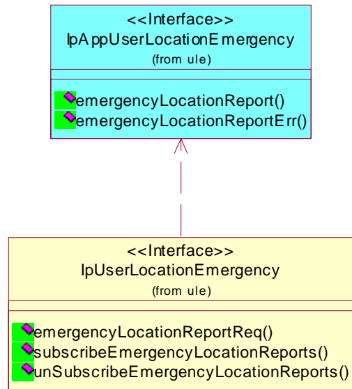
Figure: User Location Emergency Class Diagram
