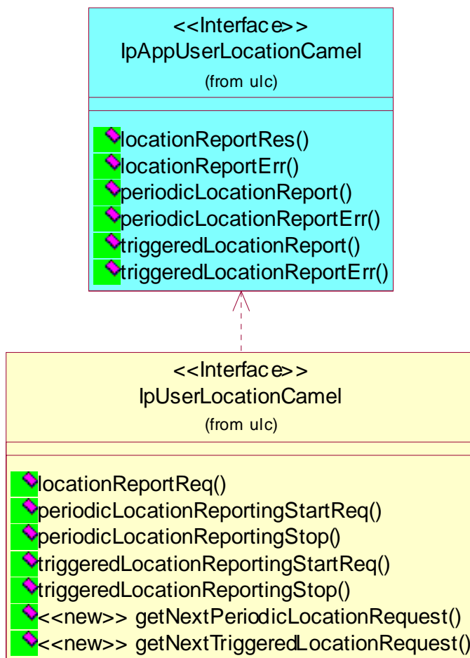
Figure: User Location Camel Class Diagram
