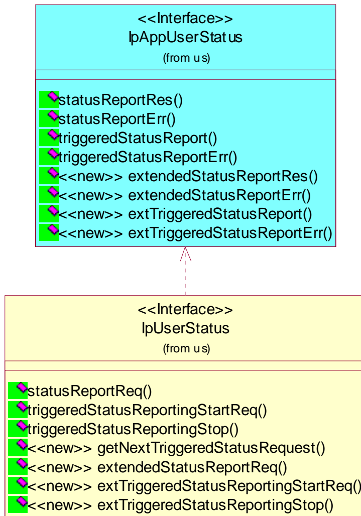
Figure: User Status Class Diagram
