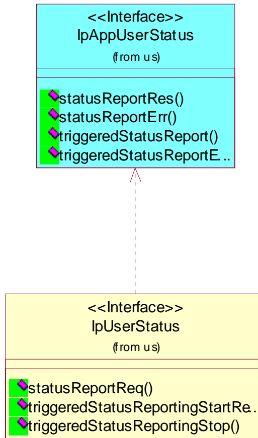
Figure: User Status Class Diagram
