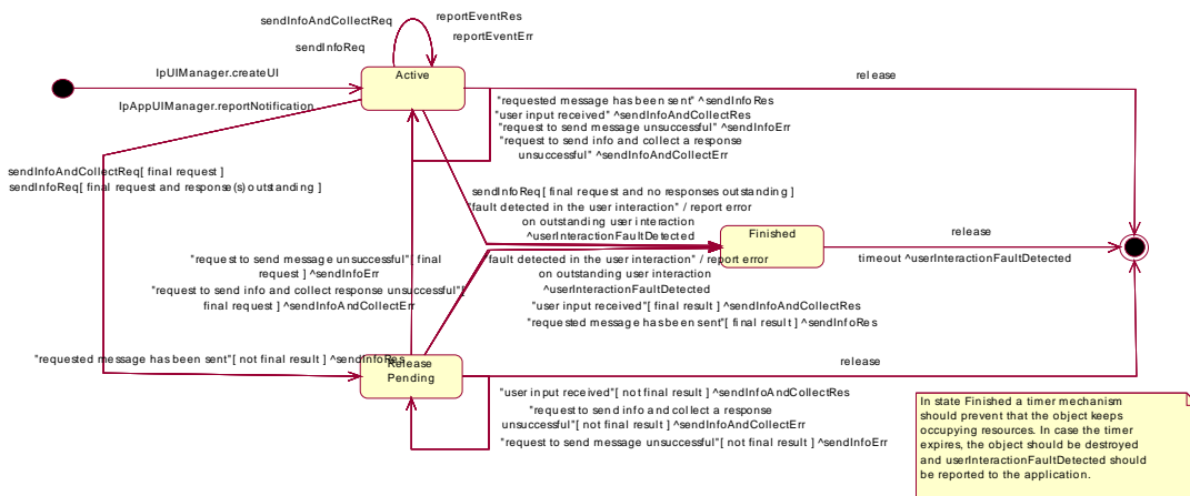
Figure : Application view on the UI object
