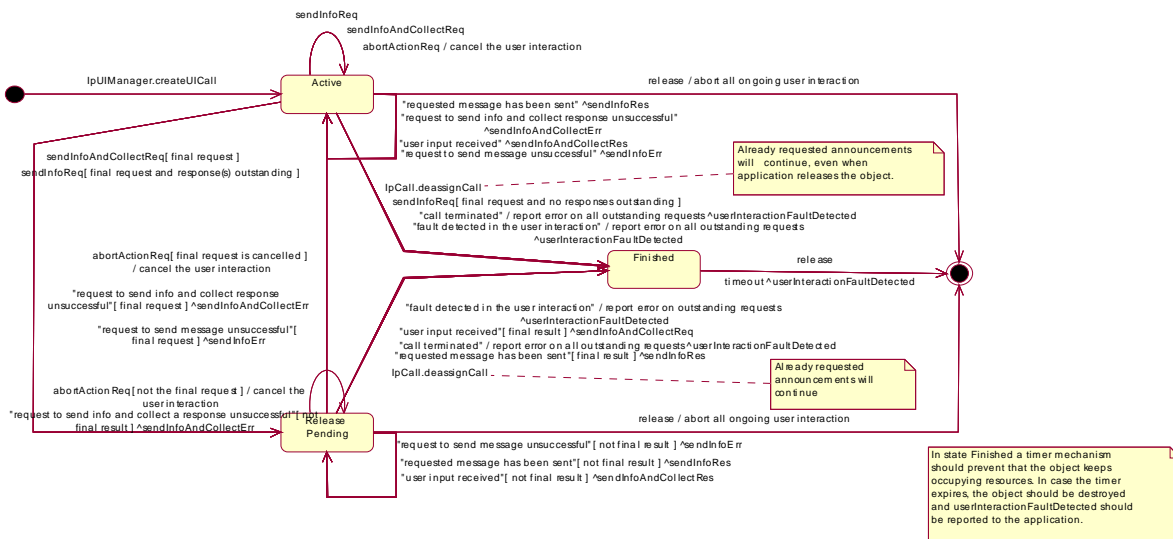
Figure : Application view on the UICall object
