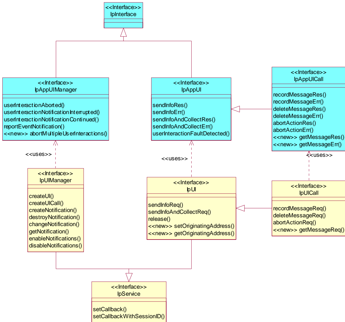
Figure: Generic User Interaction Package Overview
