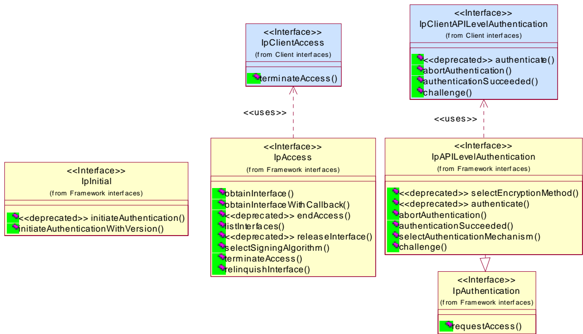
Figure: Trust and Security Management Package Overview
