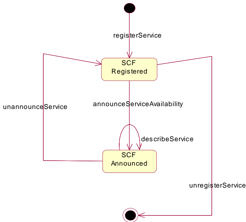
Figure : State Transition Diagram for IpFwServiceRegistration
