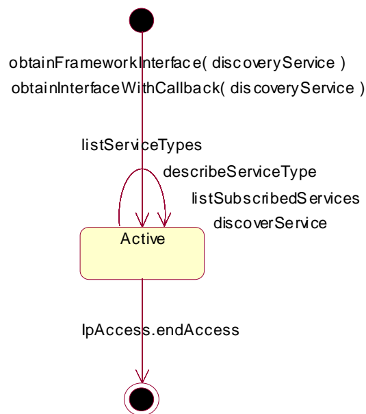
Figure : State Transition Diagram for IpServiceDiscovery
