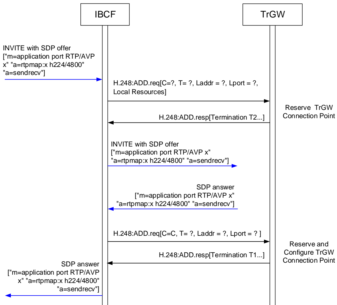
Figure 10.2.23.2.2.1: Procedure to indicate Video ROI using FECC
