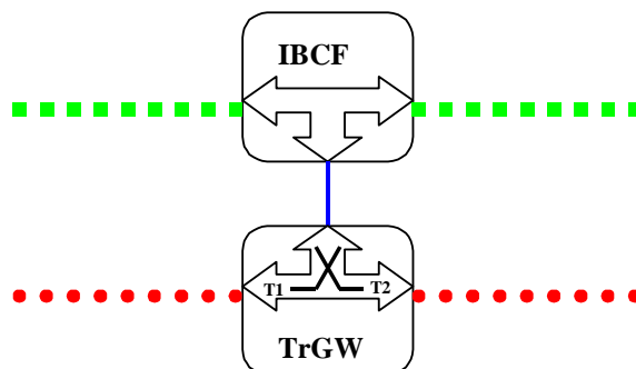
Figure 10.1.2.1: Network model
