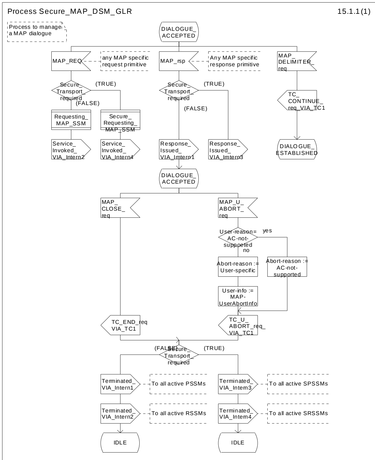
Figure 15.1/1: Process Secure_MAP_DSM_GLR
