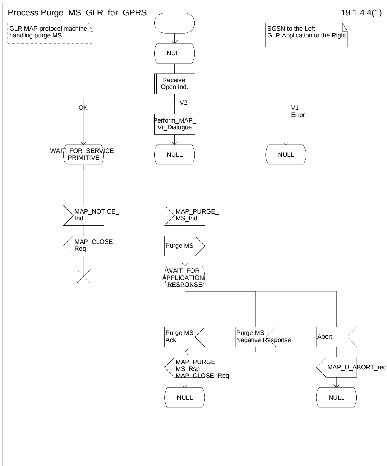
Figure 19.1.4/4: Process Purge_MS_GLR_for_GPRS
