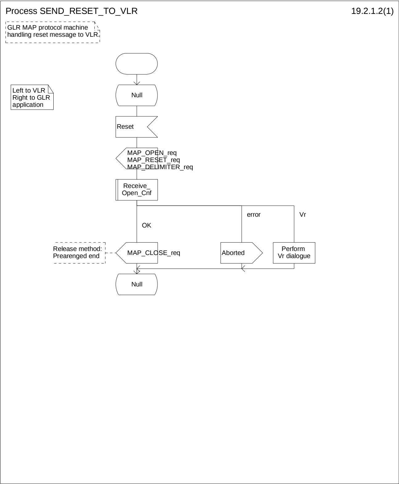
Figure 19.2.1/2: Process SEND_RESET_TO_VLR
