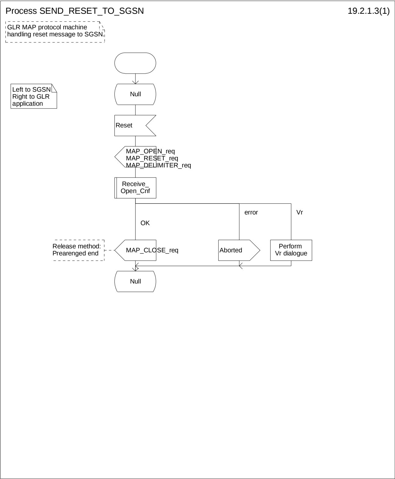
Figure 19.2.1/3: Process SEND_RESET_TO_SGSN
