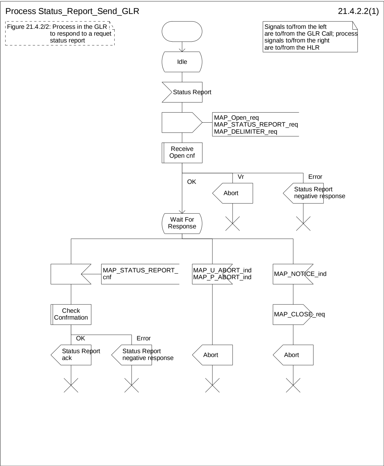
Figure 21.4.2/2: Process Status_Report_Send_GLR
