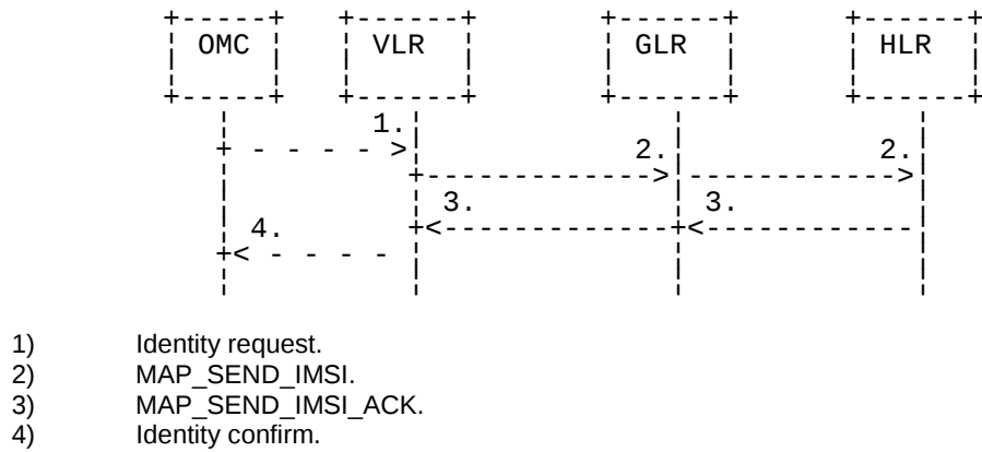
Figure 20.3/1: The subscriber identity procedure
