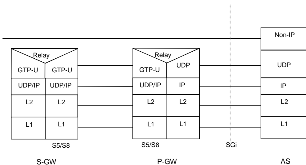
Figure 11.8: Protocol configuration for Non-IP data (user plane) using PtP tunneling
