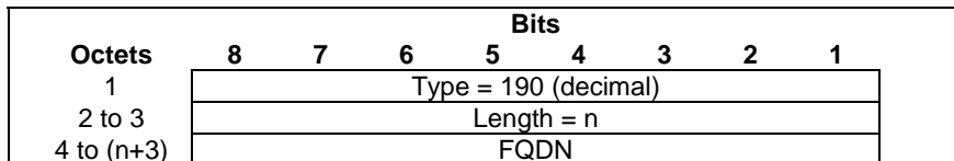
Figure 7.7.90.1: Fully Qualified Domain Name (FQDN)
