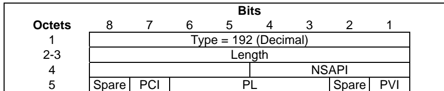
Figure 7.7.92.1: Evolved Allocation/Retention Priority II Information Element
