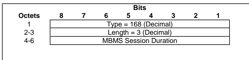
Figure 7.7.59.1: MBMS Session Duration Information Element
