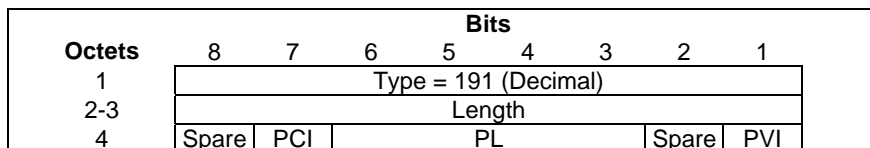
Figure 7.7.91.1: Evolved Allocation/Retention Priority I Information Element
