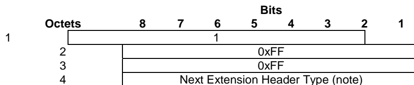
Figure 7: Suspend Request Extension Header
