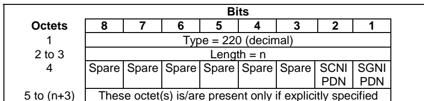
Figure 7.7.120-1: CIoT Optimizations Support Indication
