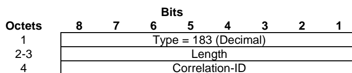
Figure 7.7.82.1: Correlation-ID Information Element
