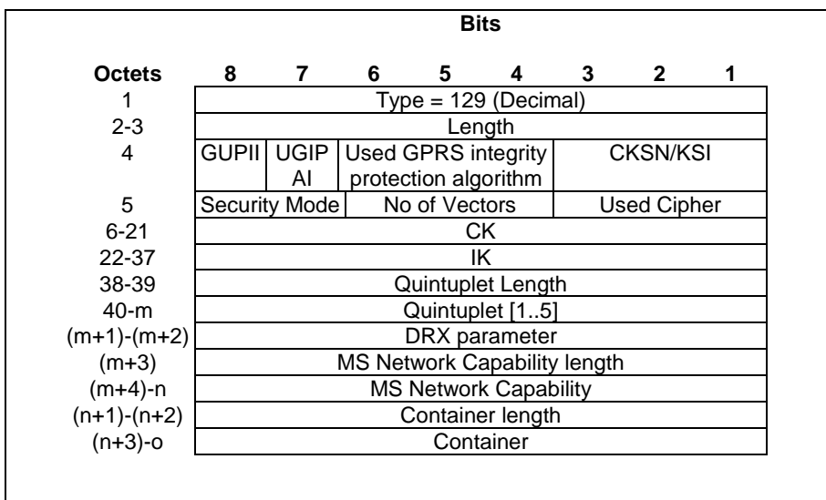
Figure 42A: MM Context Information Element with Used Cipher value, UMTS Keys and Quintuplets
