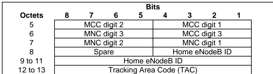
Figure 7.7.112-3: eNodeB ID for Type Home eNodeB
