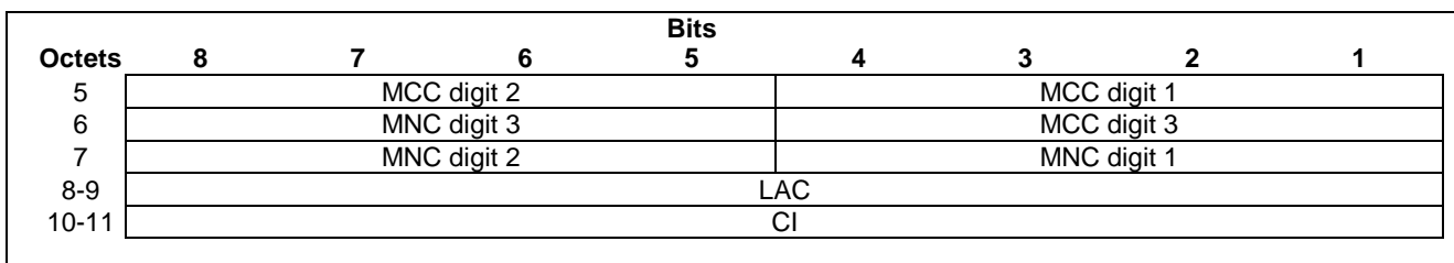
Figure 7.7.51.2: Geographic Location field for CGI
