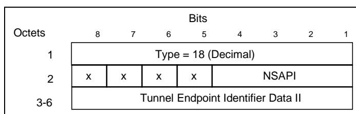
Figure 23: Tunnel Endpoint Identifier Data II Information Element
