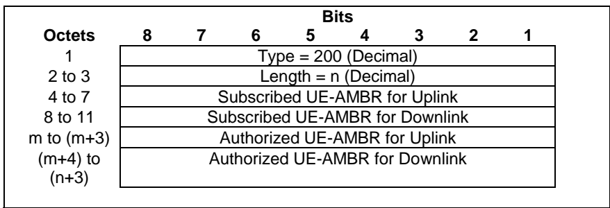
Figure 7.7.100: UE-AMBR Information Element
