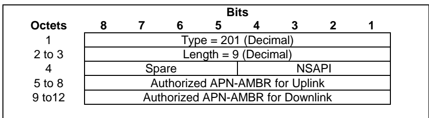
Figure 7.7.101: APN-AMBR with NSAPI Information Element
