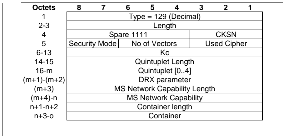
Figure 42: MM Context Information Element with GSM Keys and UMTS Quintuplets
