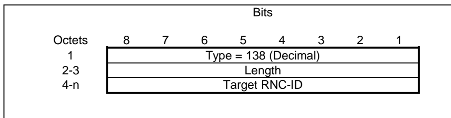
Figure 51: Target Identification Information Element
