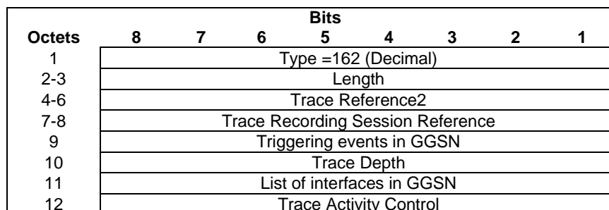
Figure 7.7.62.1: Additional Trace Info Information Element
