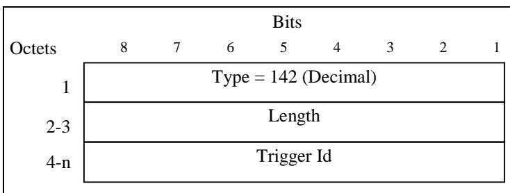
Figure 56: Trigger Id Information Element
