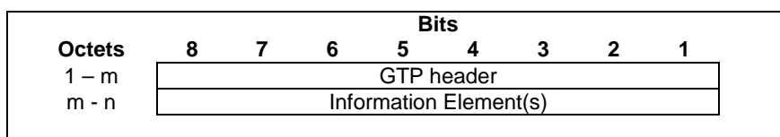
Figure 64: GTP Header followed by subsequent Information Elements
