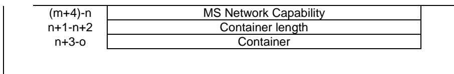
Figure 42: MM Context Information Element with GSM Keys and UMTS Quintuplets
