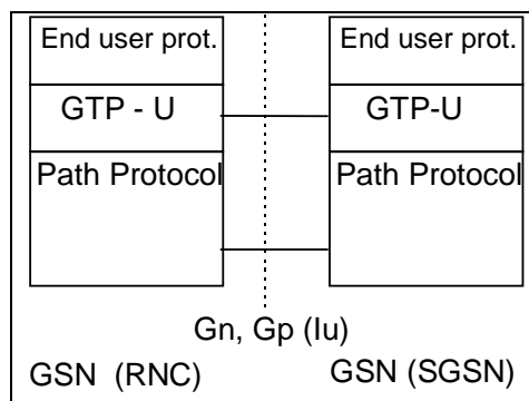
Figure 65: GTP-U - Protocol Stack (GTP-U over the lu in brackets)
