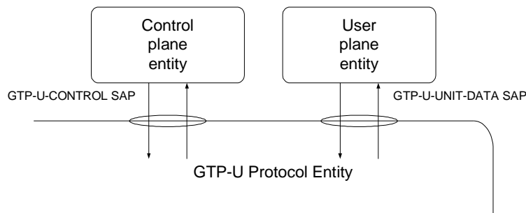
Figure 64: The GTP-U-Control SAP and GTP-U-DATA SAP
