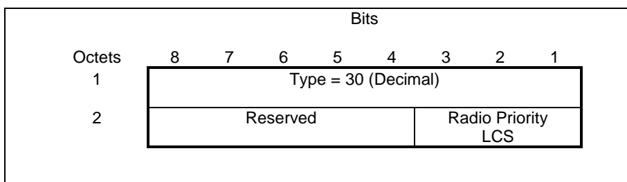
Figure 33b: Radio Priority LCS Information Element
