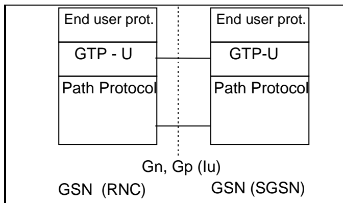
Figure 65: GTP-U - Protocol Stack (GTP-U over the lu in brackets)
