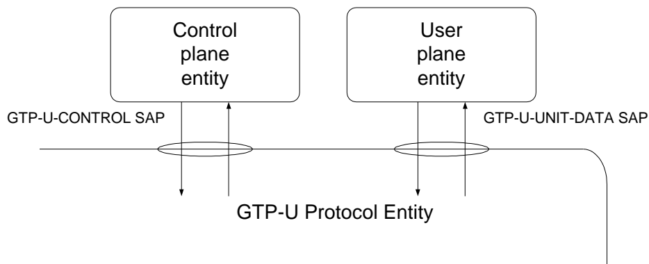
Figure 64: The GTP-U-Control SAP and GTP-U-DATA SAP
