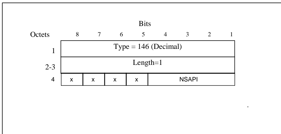
Figure 60b: Additional RAB Setup Information IE for release of resources
