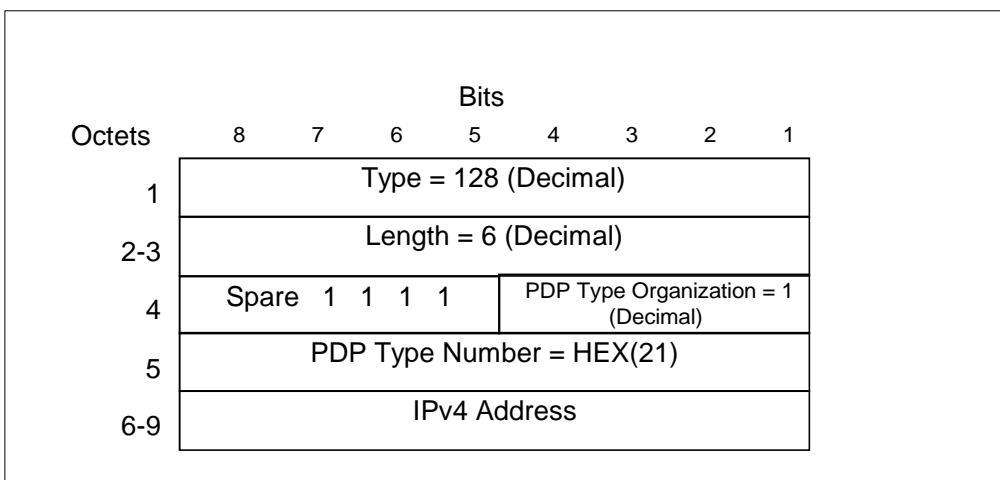
Figure 36: End User Address Information Element for IPv4
