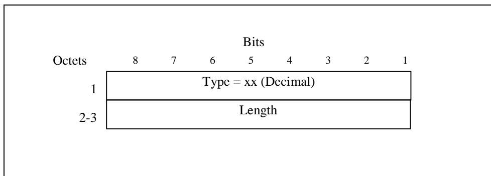
Figure 60 : PDP Context Prioritization Information Element
