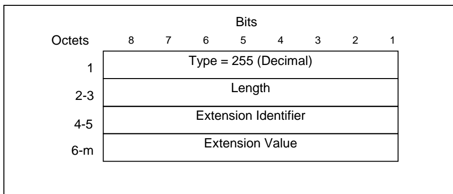
Figure 61: Private Extension Information Element
