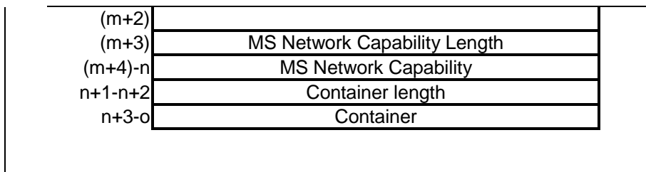
Figure 42: MM Context Information Element with GSM Keys and UMTS Quintuplets
