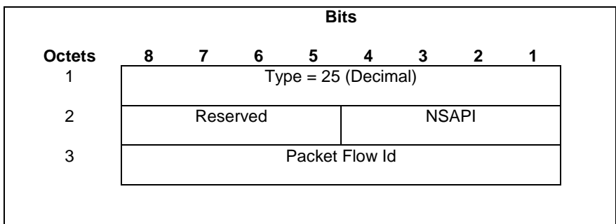
Figure 30: Packet Flow Id Information Element
