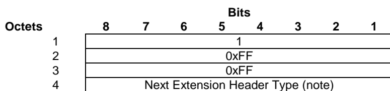
Figure 7: Suspend Request Extension Header
