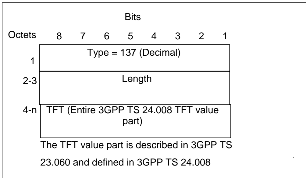
Figure 50: Traffic Flow Template Information Element
