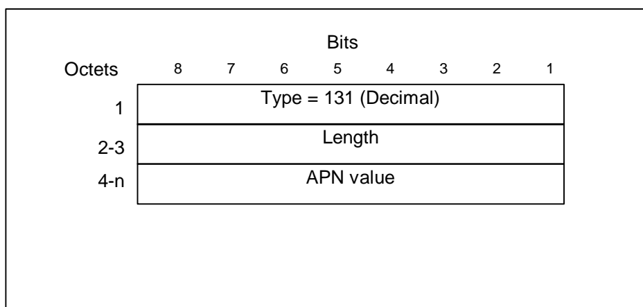
Figure 44: Access Point Name Information Element
