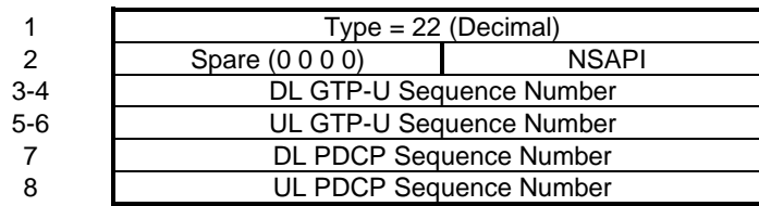
Figure 27: RAB Context Information Element
