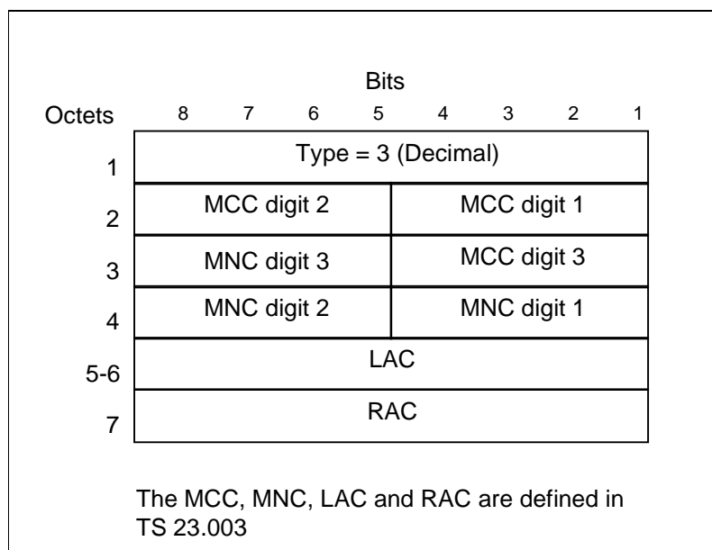
Figure 11: RAI Information Element
