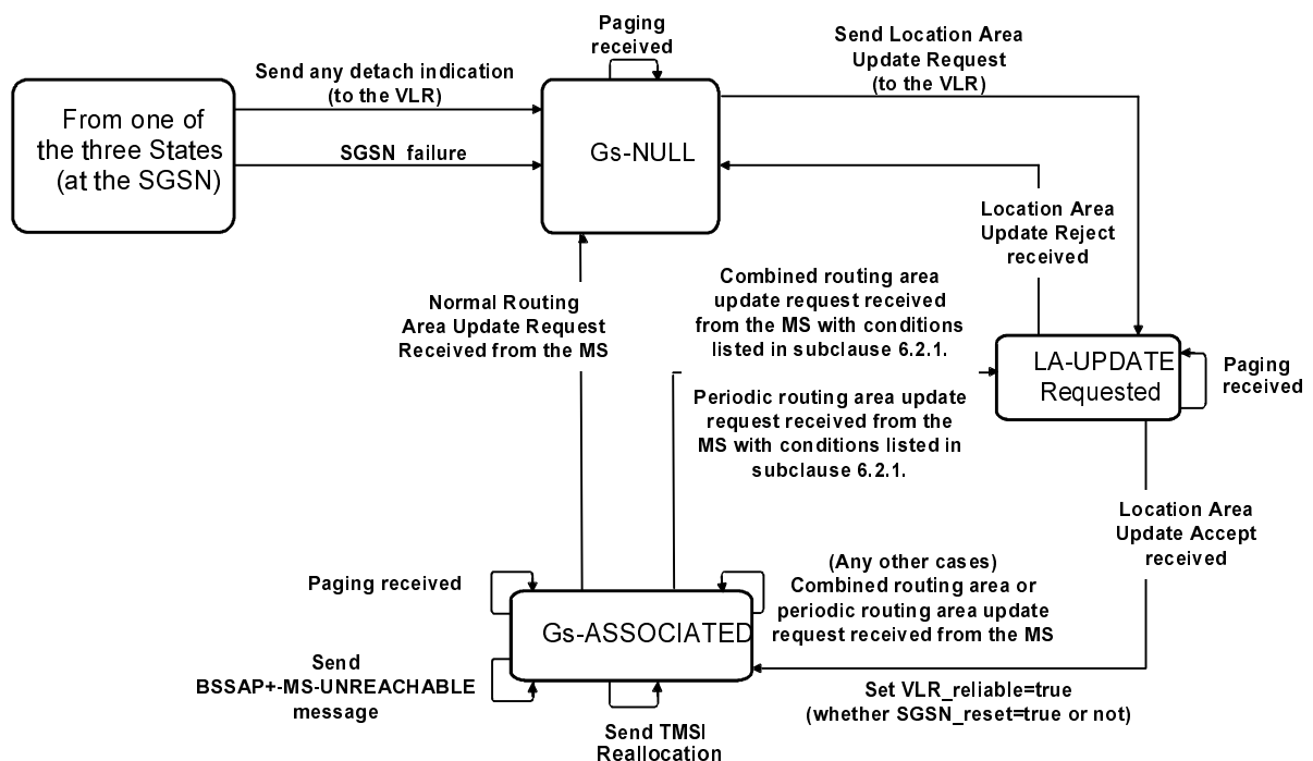
Figure 4.2/3GPP TS 29.018: State diagram at the SGSN
