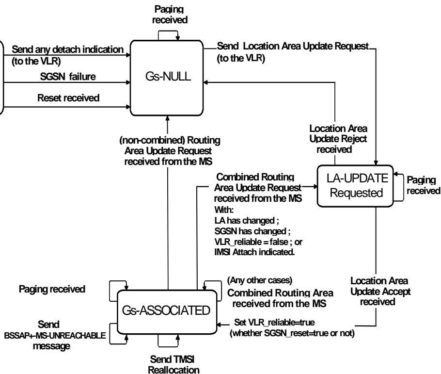
Figure 4.2/3GPP TS 29.018: State diagram at the SGSN
