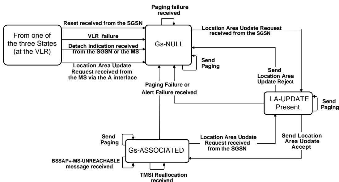
Figure 4.1/3GPP TS 29.018: State diagram at the VLR
