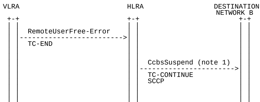
Figure 6.4: Signalling flow for CCBS Suspend Invocation (RemoteUserFree_Result)
