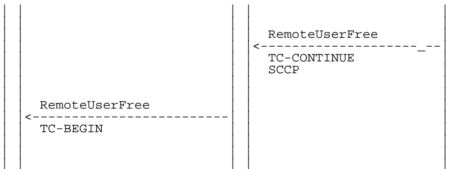
Figure 6.3: Signalling flow for Remote User Free Invocation
