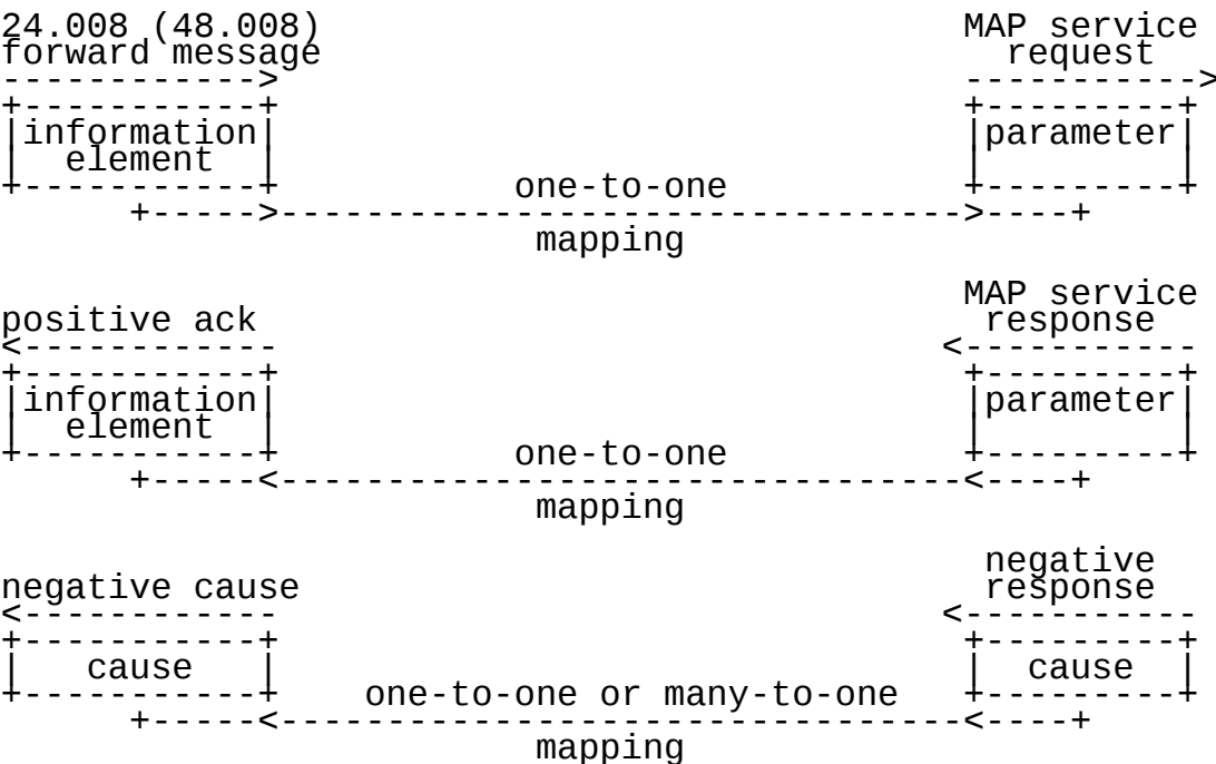
Figure 1: Illustration of mapping principles in the MSC
