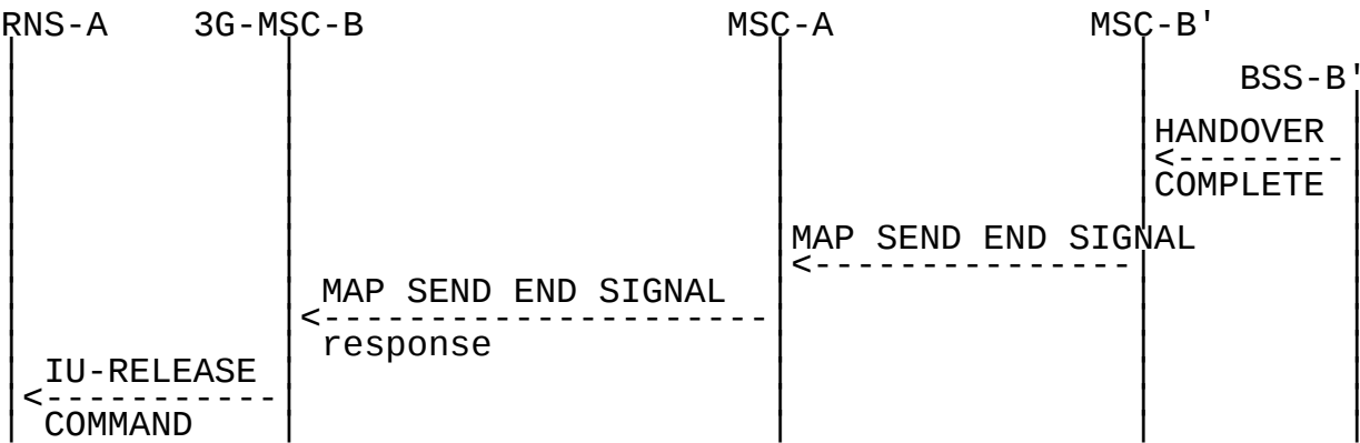
Figure 35: Signalling for Subsequent Inter-MSC Handover to third MSC (MSC-B') completion (Successful completion of the procedure)
