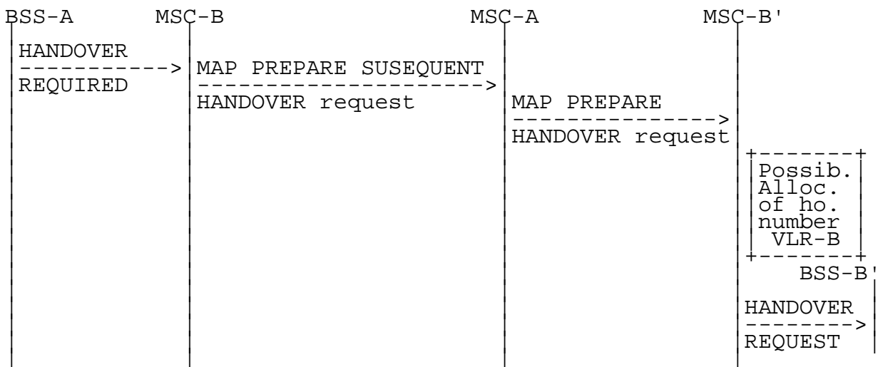
Figure 16: Signalling for Subsequent Inter-MSB Handover to third MSB (MSB-B') initiation
