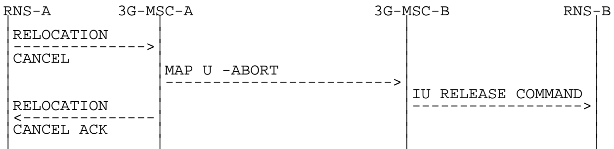
Figure 51: Signalling for Basic Inter-MSA Relocation execution (Negative outcomes)
