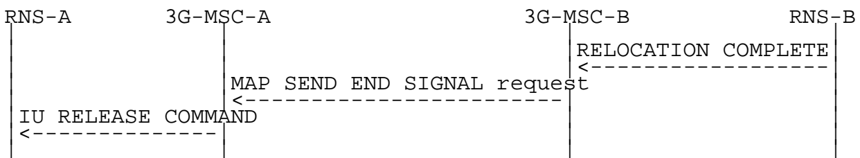
Figure 52: Signalling for Basic Inter-MSA Relocation completion
