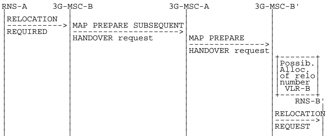
Figure 60: Signalling for Subsequent Inter-MSR Relocation to third MSR (3G_MSC-B') initiation
