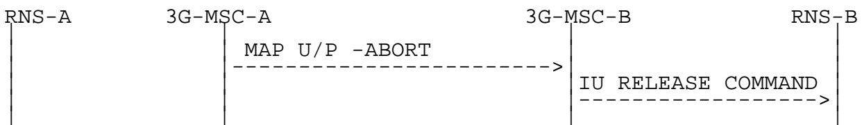
Figure 54: Signalling for Basic Inter-MSA Relocation completion (Negative outcome)
