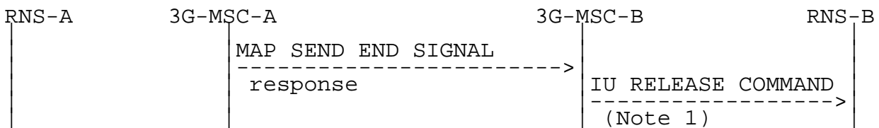
Figure 53: Signalling for Basic Inter-MSA Relocation completion (Positive outcome)
