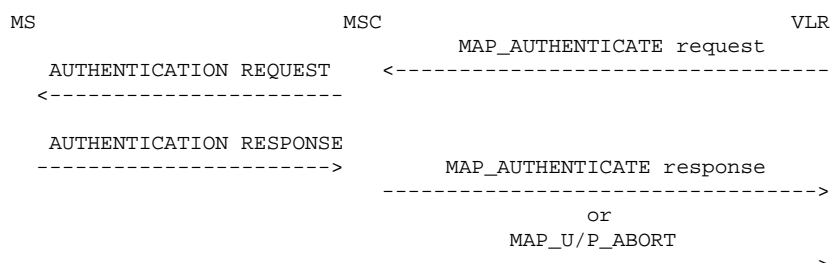
Figure 2: Authentication operation
