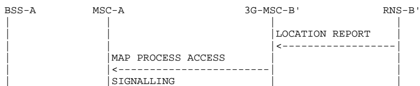
Figure yy: Signalling for updating of anchor MSC after change of location in RNS
