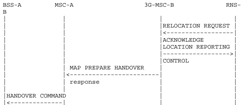
Figure 38: Signalling for Basic Inter-MSC Handover execution (Positive outcome)
