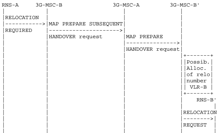
Figure 60: Signalling for Subsequent Inter-MSR Relocation to third MSR (3G_MSR-B') initiation
