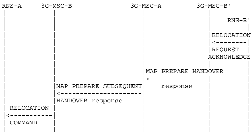
Figure 61: Signalling for Subsequent Inter-MSR Relocation to third MSR (3G_MSR-B') execution (Positive outcome)
