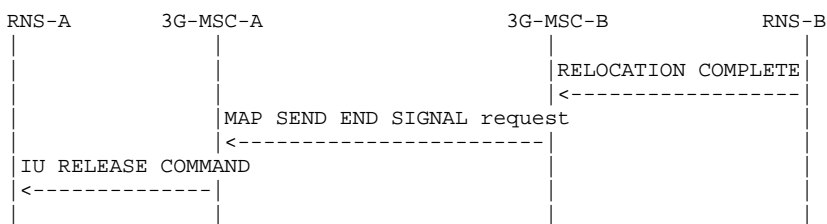
Figure 52: Signalling for Basic Inter-MSA Relocation completion
