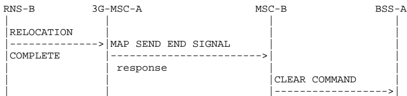
Figure 46: Signalling for Subsequent Inter-MSC Handover back to 3G_MSC-A completion (Successful completion of the procedure)
