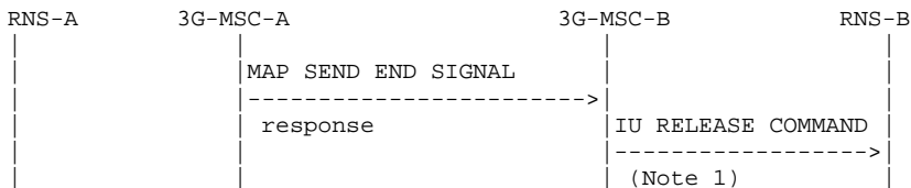
Figure 53: Signalling for Basic Inter-MSA Relocation completion (Positive outcome)
