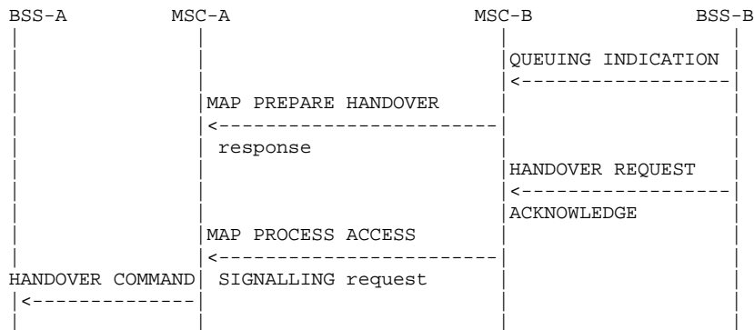
Figure 6: Signalling for Basic Inter-MSC Handover execution (Positive outcomes)
