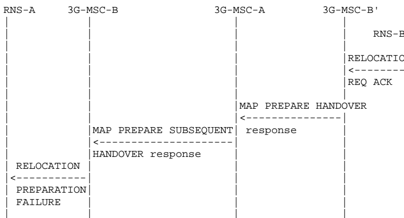
Figure 62: Signalling for Subsequent Inter-MSC Relocation to third MSC (3G_MSC-B') execution (Negative outcome)
