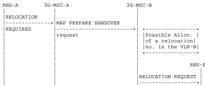
Figure 50a: Signalling for Basic Inter-MSC Relocation initiation (no trace related messages transferred)
