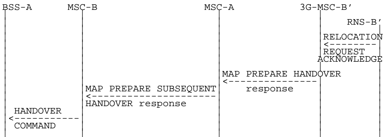
Figure 46: Signalling for Subsequent Inter-MSC Handover to third MSC (3G_MSC-B') execution (Positive outcome)
