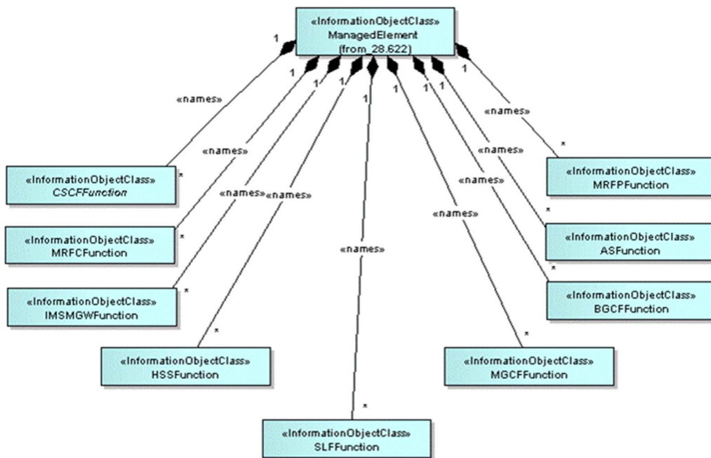
Figure 4.2.1.1: IMS NRM Containment/Naming relationships
