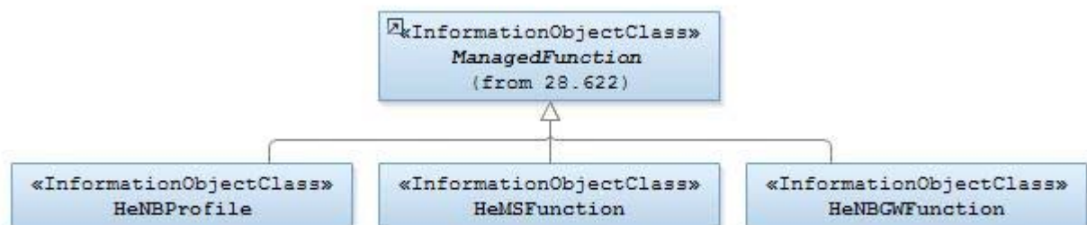
Figure 4.2.2-1: HeNS NRM Inheritance Hierarchy
