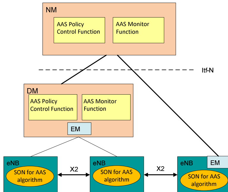
Figure 4.8.4.2-1: Example when the SON for AAS algorithm is located in the eNB(s)
