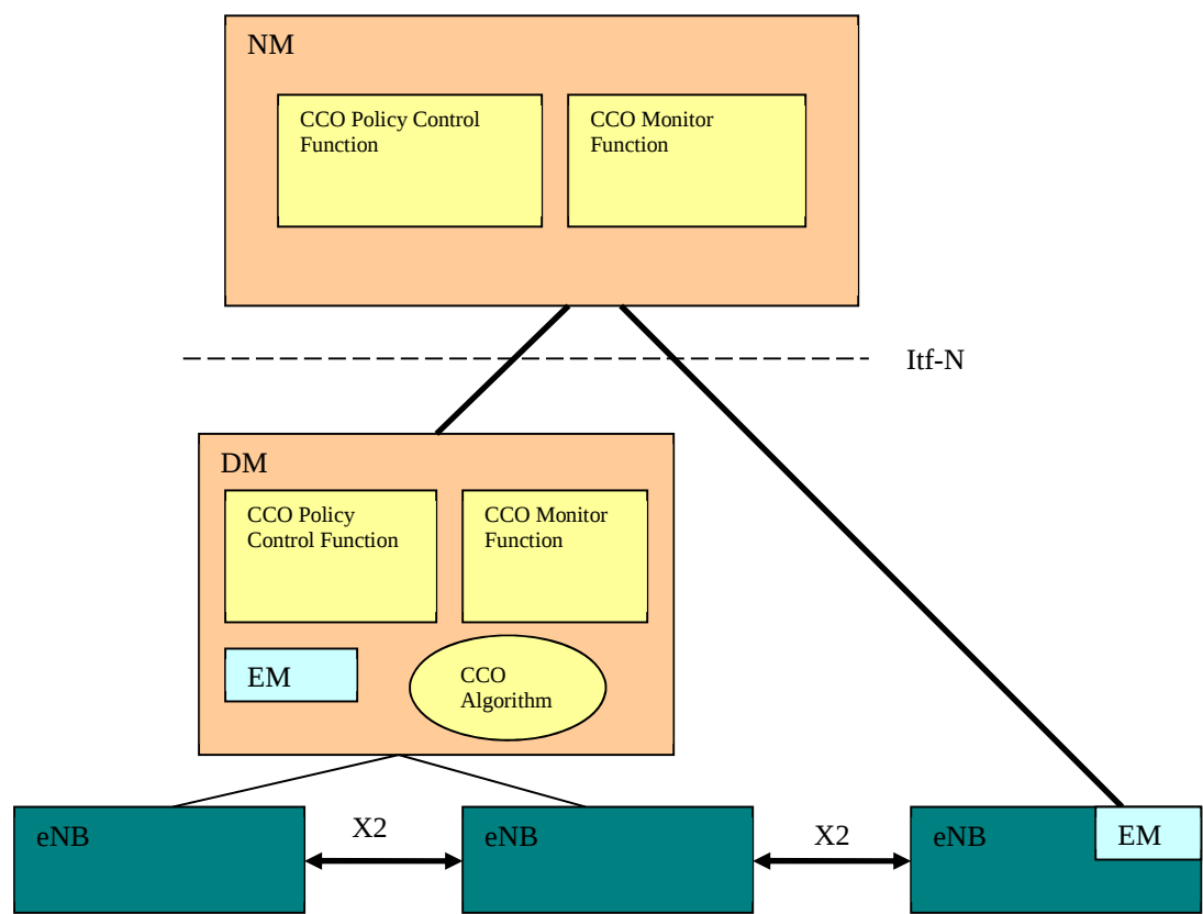
Figure 4.5.4.2-1: Example when the CCO SON algorithm is located in DM
