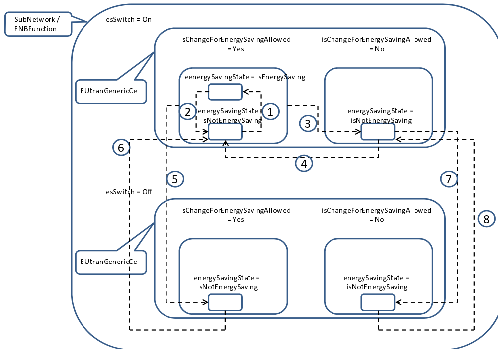
Figure C-2: State diagram for Distributed and EM-centralized ESM
