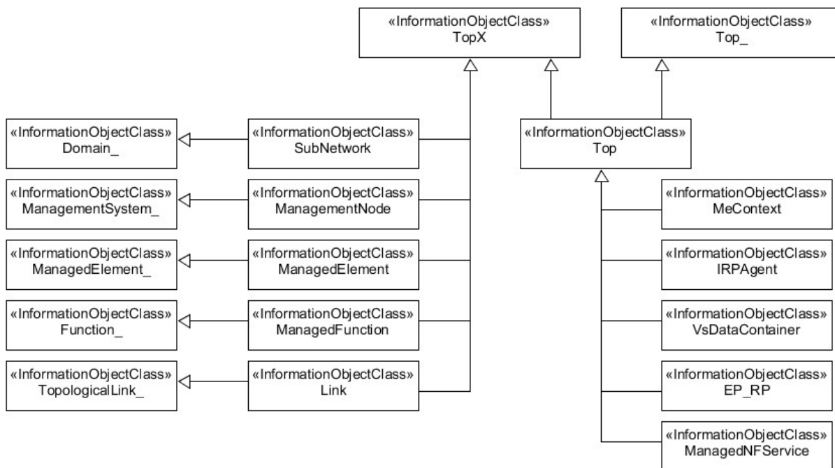
Figure 4.2.2-1: Inheritance Hierarchy NRM fragment
