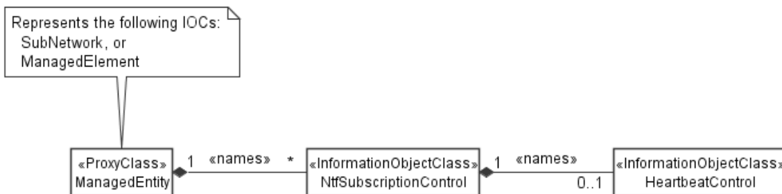
Figure 4.2.1-5: Notification subscription and heartbeat notification control NRM fragment
