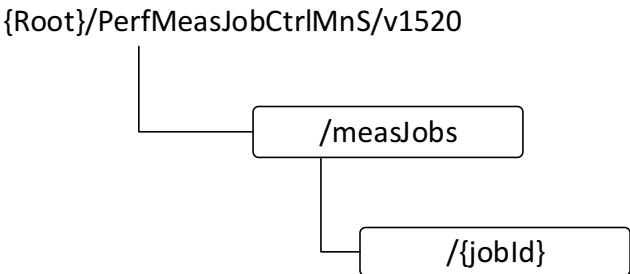
Figure 8.2.0-1: Resource URI structure of the performance measurement job control service
