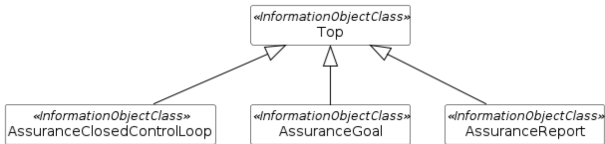
Figure 4.1.2.2.2.1: Assurance management inheritance relationships
