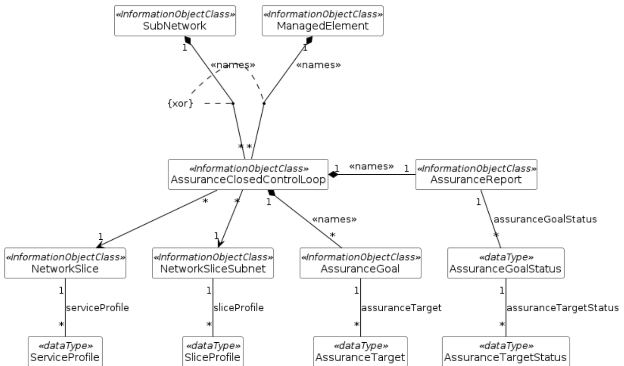
Figure 4.1.2.2.1.1: Assurance management NRM fragment
