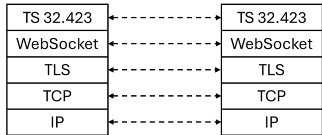
Figure 12.5.1.1.4-1: Protocol stack for streaming trace data reporting
