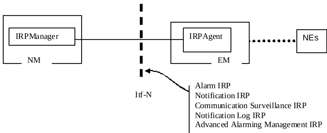
Figure 4.2-1: System Context
