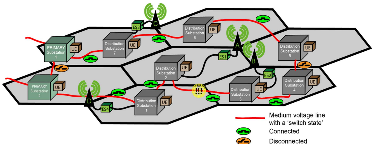
Figure C.2-2: Local failure event
