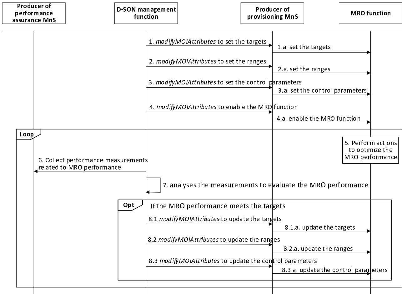
Figure 8.2.2-1: MRO procedure
