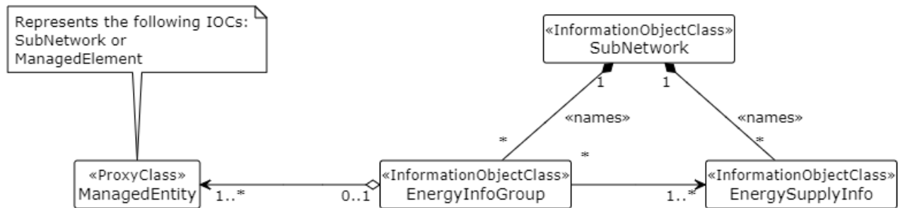
Figure 8.2.1-1: Energy information NRM fragment
