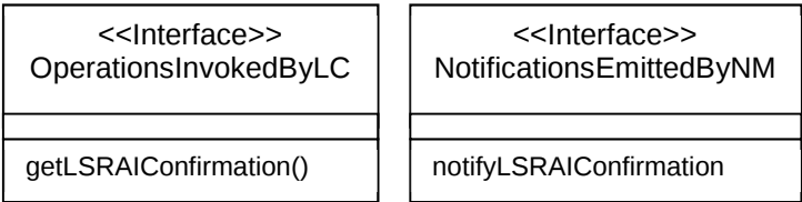
Figure 6.1.1-2: Class diagram representing the interface OperationsInvokedByLC and the interface NotificationsEmittedByNM (scenario 1)
