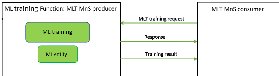
Figure 6.2.2.1-1: ML training requested by MLT MnS consumer
