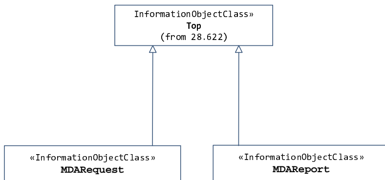
Figure 9.2.2-1: Inheritance Hierarchy
