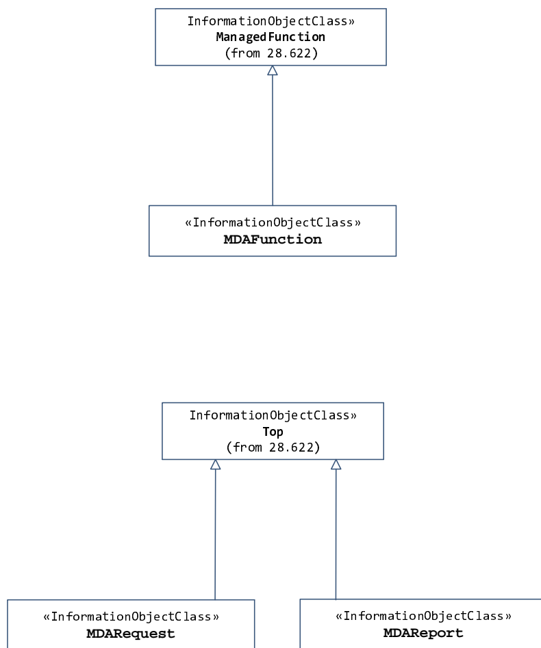
Figure 9.2.2-1: Inheritance Hierarchy
